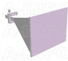
LB-112-20-C-TFSPO Standard Gain Horn Antenna 7.05-10GHz 20dB Gain TNC Female
