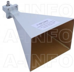
LB-112-20-C-TF Standard Gain Horn Antenna 7.05-10GHz 20dB Gain TNC Female
